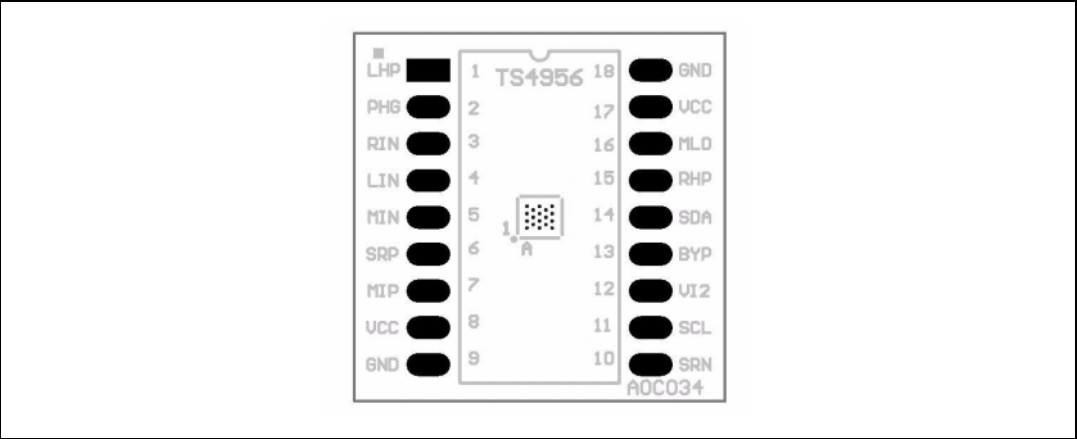
Figure 5. TS4956 DEMO BOARD top view
